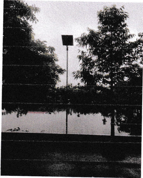
Solar System
